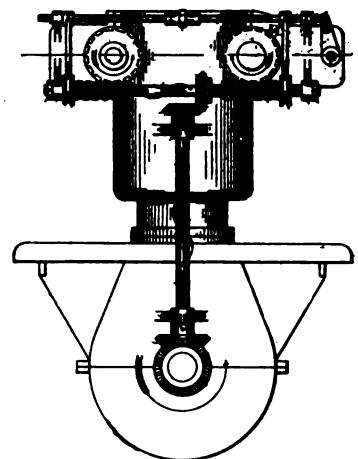
Mead Engine with Rotary Valves.
